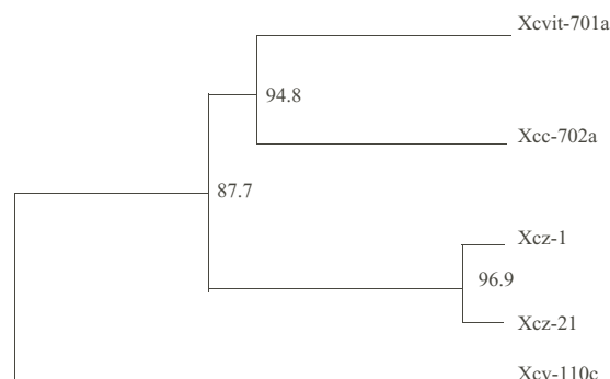
Figure 3. Dendrogram estimated phylogenetic relationships based on sequences similarity in the 16S–23S rDNA spacer regions of X. campestris pv. zinniae strains Xcz-1 and Zcz-21, X. axonopodis pv. vesicatoria Xcv-110c, X. hortorum pv. vitians Xcvit-701a and X. campestris pv. campestris Xcc-702a.
